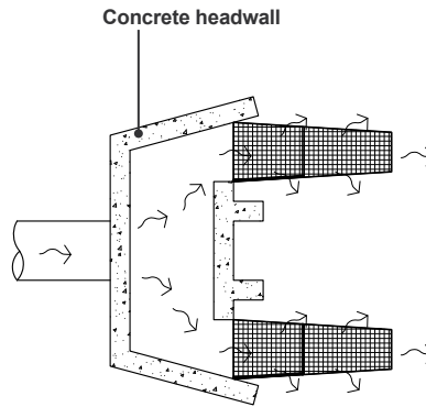
FIXED TO CONCRETE HEADWALL DUAL UNIT
